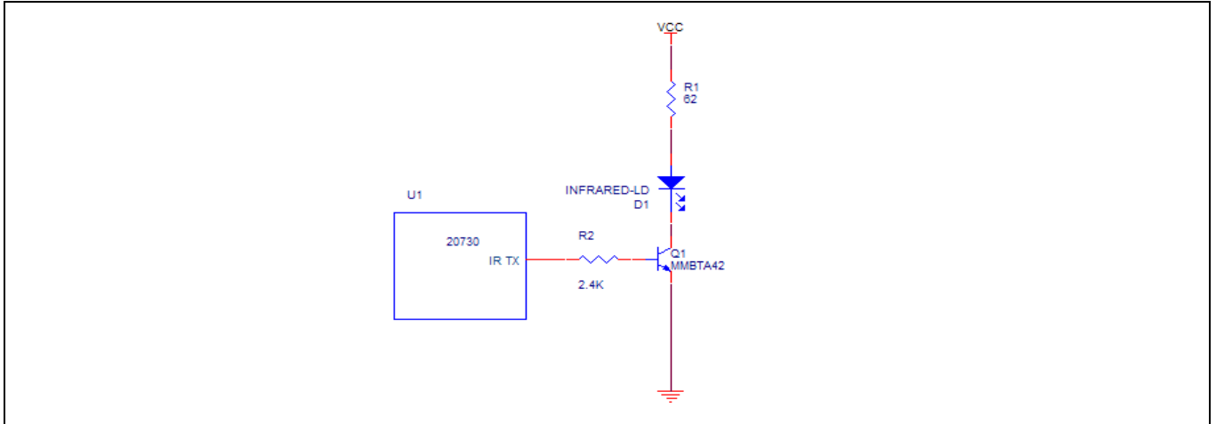
Figure 2 Infrared TX
