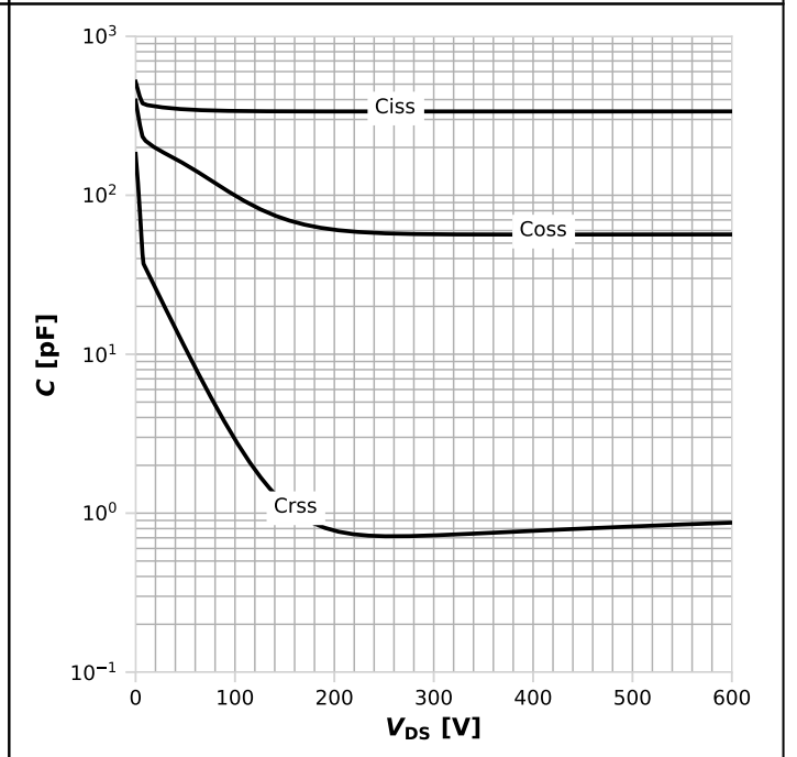
Diagram 18: Typ. capacitances
